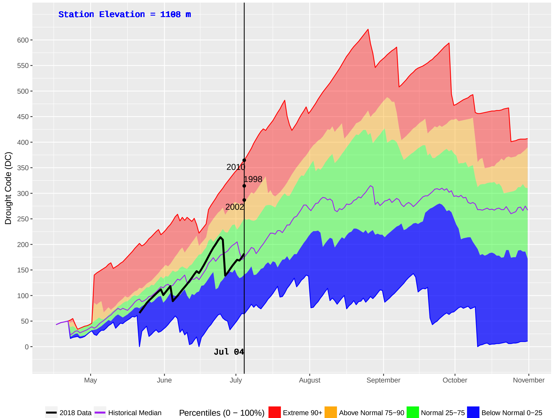
NABESHE (151) : Historical (1987–2016) and Current (2018) Noon Drought Code (DC)
